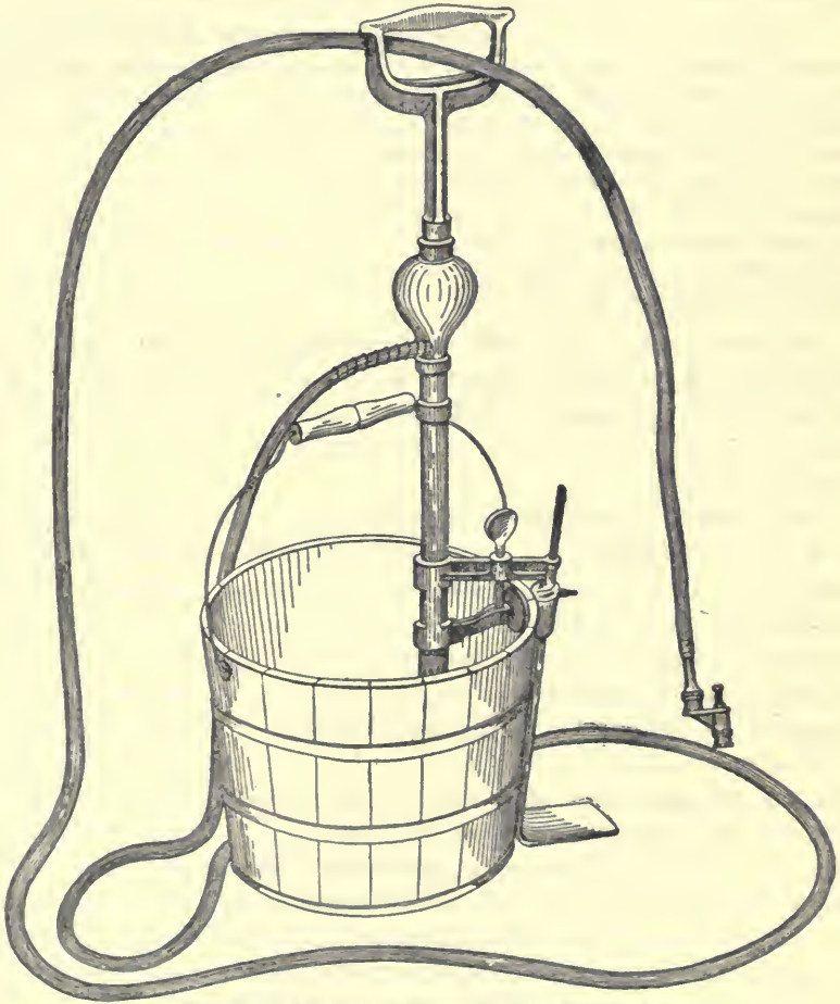
FIG. 5.—Pall spraying pump for small herds.
